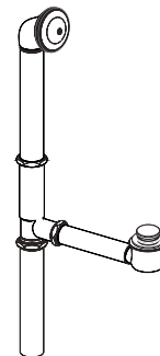
ERA™ FREESTANDING TOE-TAP DRAIN KIT (Requires purchase of GVII Gasket Kit if used on Era™ Slipper 6934)
